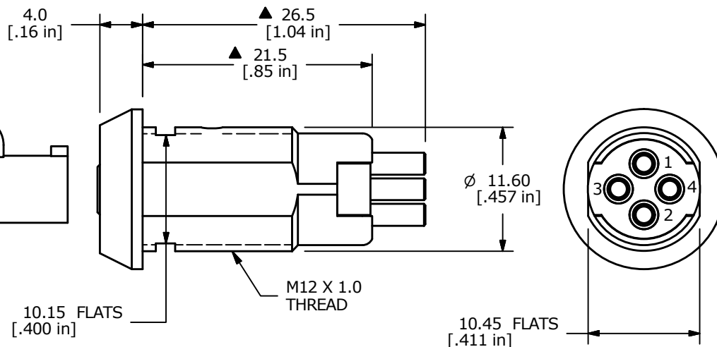
SHOWN WITH PROVIDED HEX NUT
