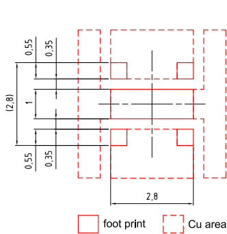
Component Location on Pad
