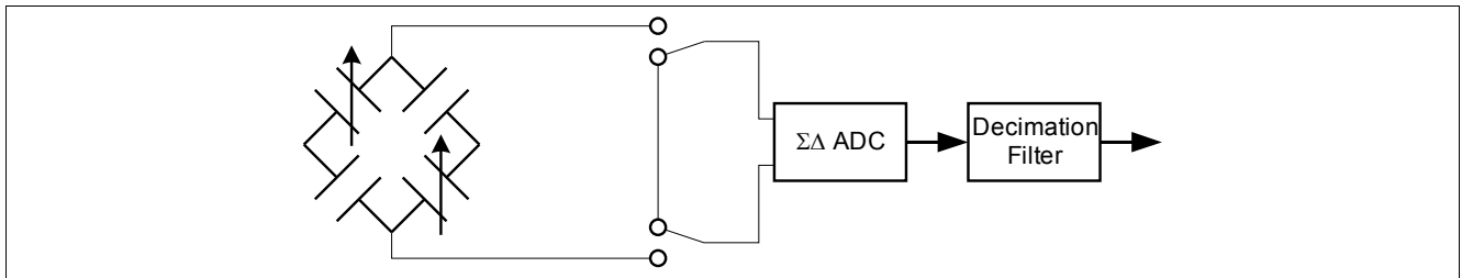
Figure 12 Diag1 functionality
