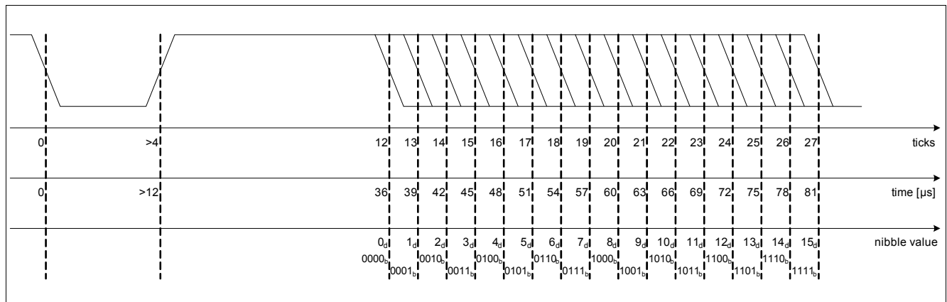
Figure 8 Nibble timing
