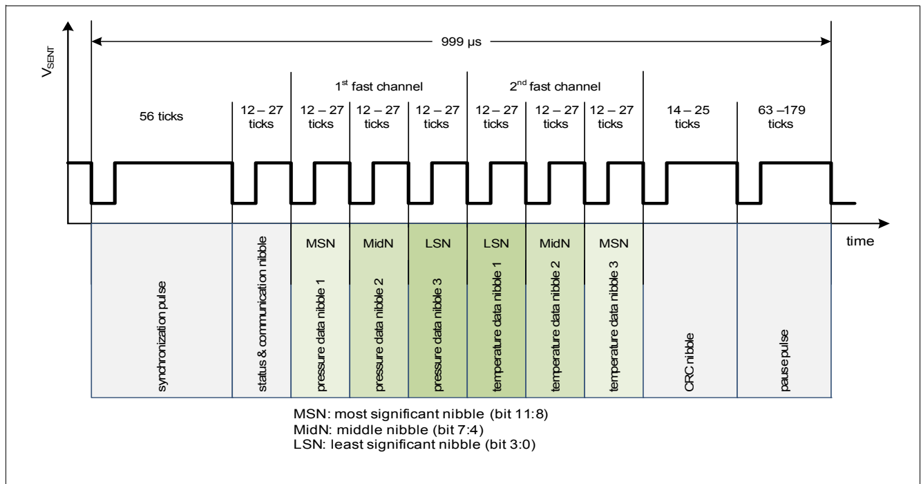
Figure 7 Message transmission
