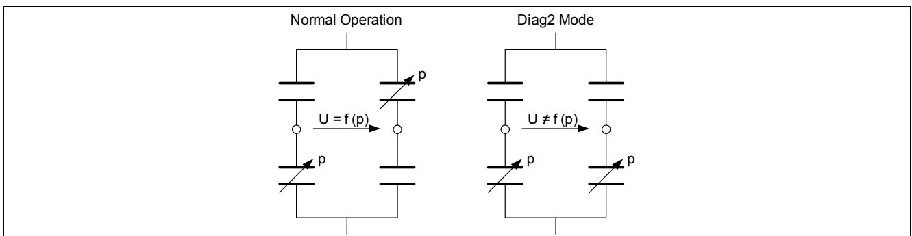
Figure 13 Diag2 functionality
