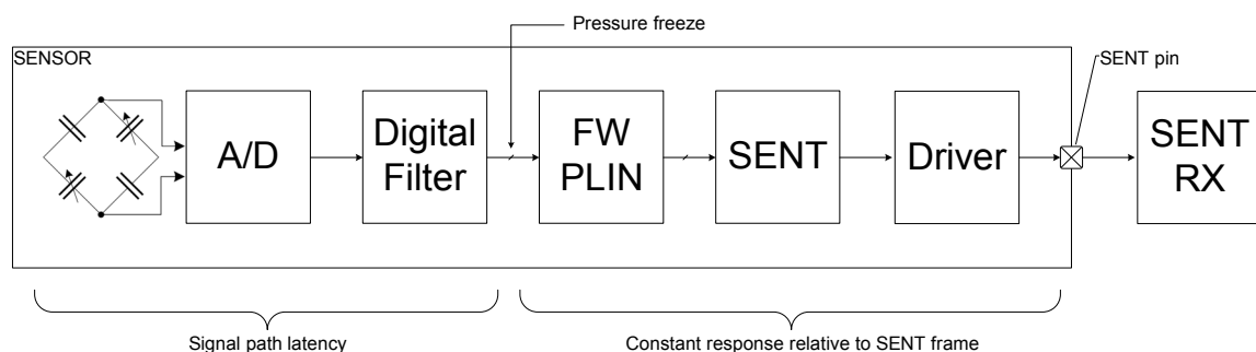
Figure 14 Pressure signal path latency t_{\text{path\_pres}} (pressure settling time)
