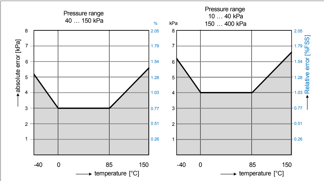
Figure 4 Accuracy for pressure acquisition
