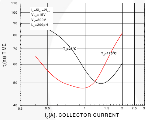
Figure 15. Inductive Switching Time, t_r
