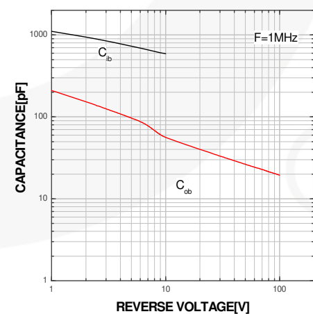
Figure 6. Capacitance
