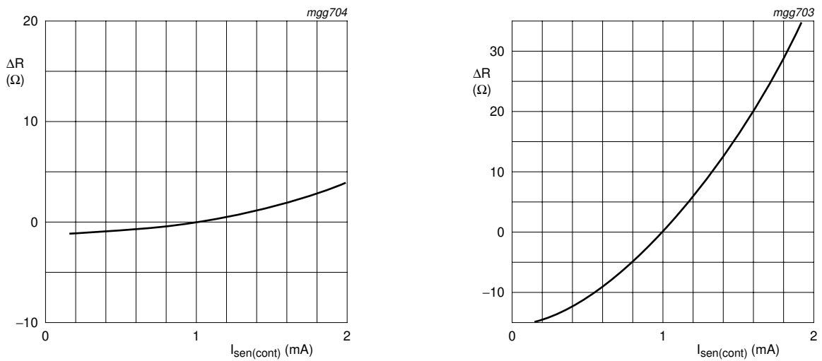
Fig 1. Sensor resistance as a function of operating current
