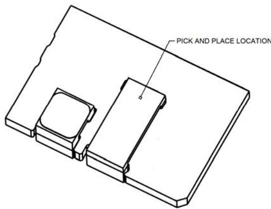
Figure 46. Pick and Place Location.
