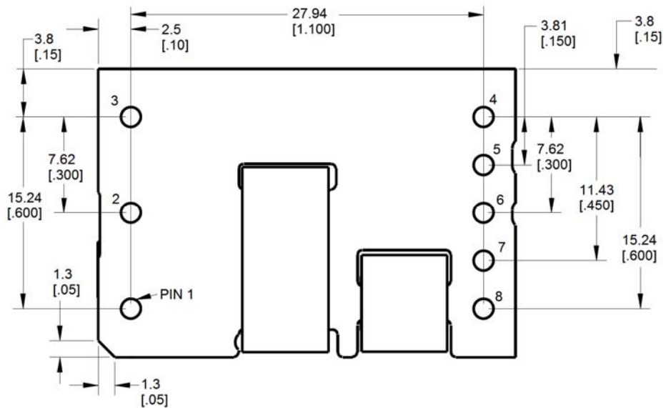
Bottom View
