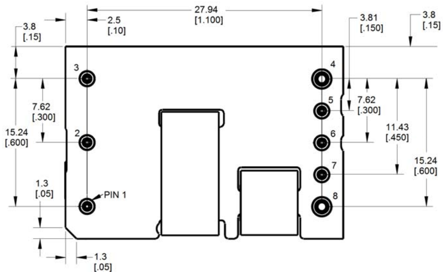
Bottom View
