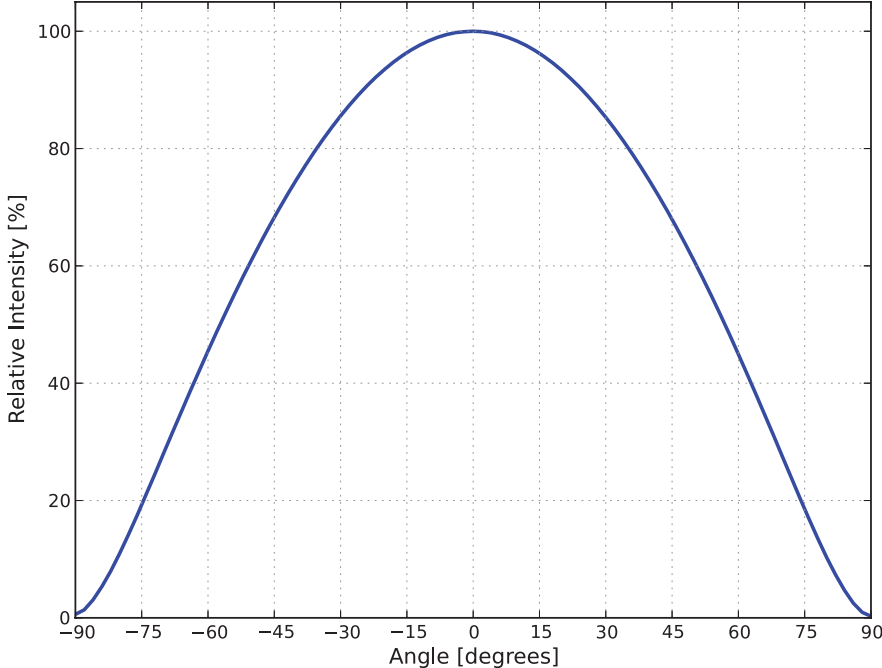
Figure 6. Typical radiation pattern for LUXEON 3535L Color Line at 100mA, T_j=25^{\circ}\text{C} .
