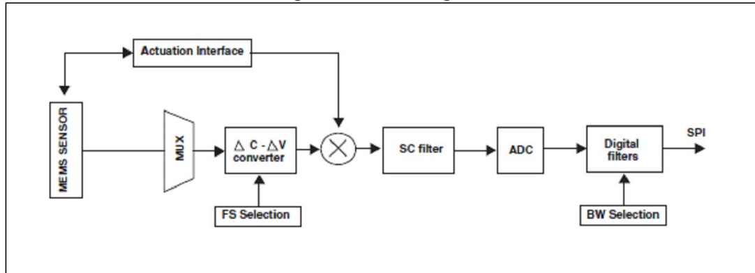
Figure 1. Block diagram
