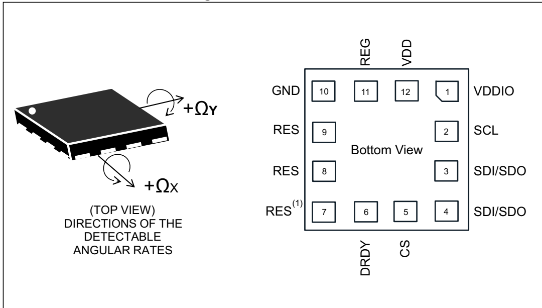
Figure 2. Pin connections
