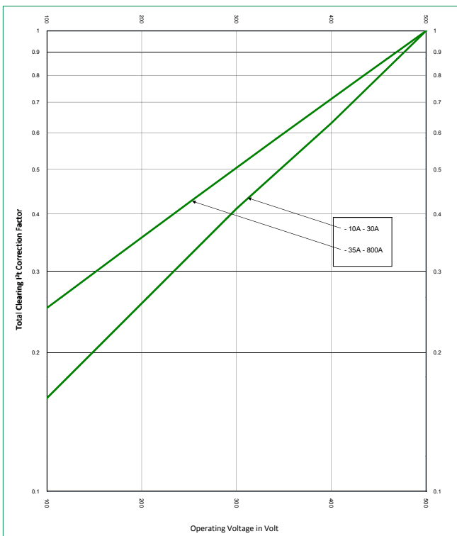
Total Clearing I²t Correction Factor Curve
