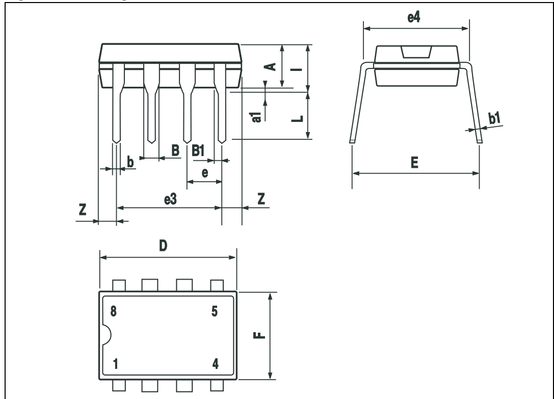
Figure 31. Package dimensions
