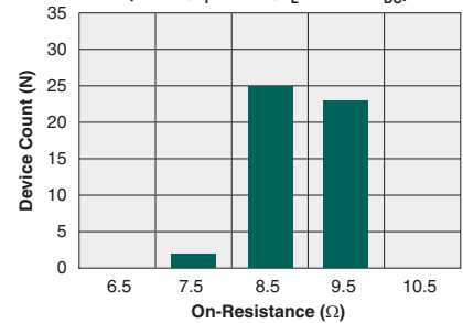
Typical On-Resistance Distribution (N=50, I_F=5\text{mA} , I_L=170\text{mA}_{DC} )
