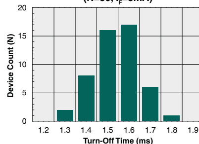
Form-B Typical Turn-Off Time (N=50, I_F=5mA )
