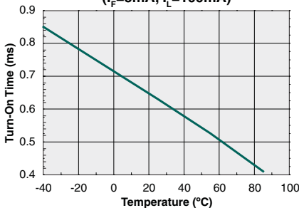
Form-B Typical Turn-On Time vs. Temperature ( I_F=5mA , I_L=100mA )
