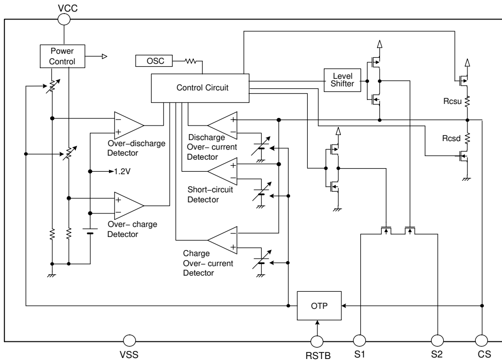
Figure 3. Block Diagram
