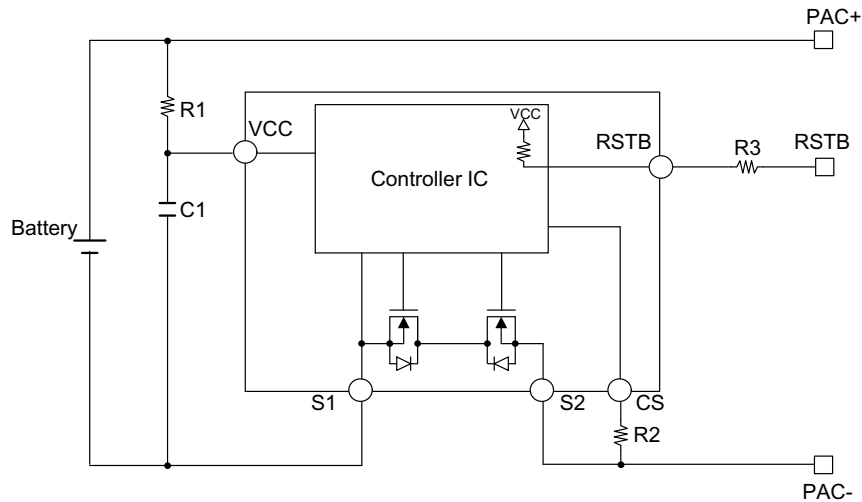
Figure 1. Example of Application Circuit
