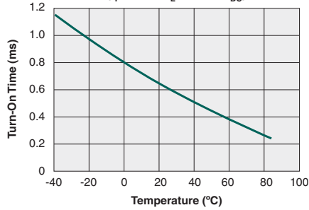
Typical Turn-On Time vs. Temperature ( I_F=5\text{mA} , I_L=170\text{mA}_{DC} )
