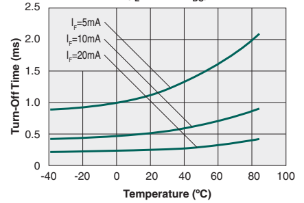
Typical Turn-Off Time vs. Temperature ( I_L=170\text{mA}_{DC} )
