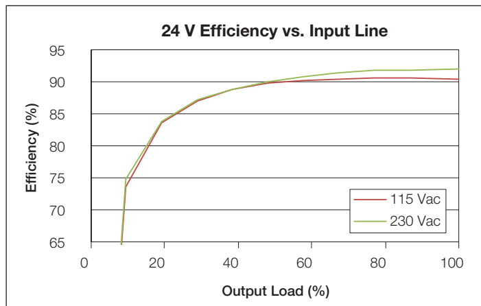
Fig 8. 24 V Efficiency Curve
