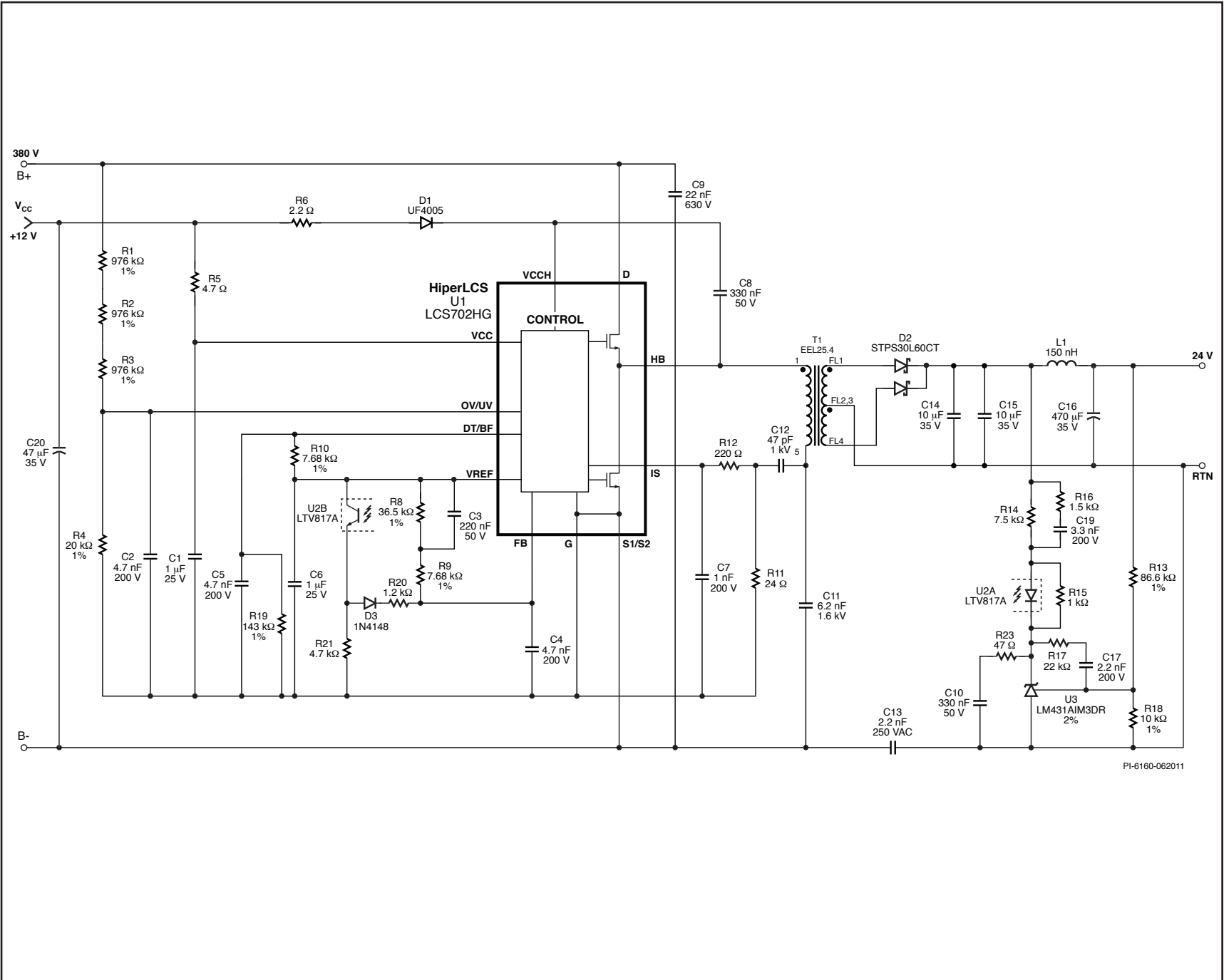
Figure 4. 150 W Laser-Jet Printer Power Supply.
