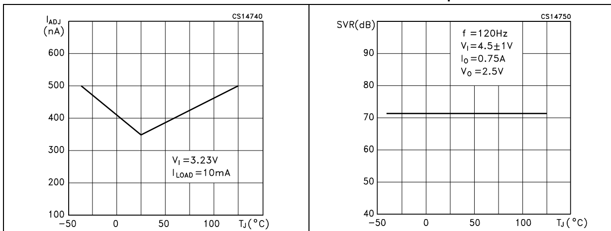
Figure 15. Adjust pin current vs. temperature Figure 16. Supply voltage rejection vs. temperature
