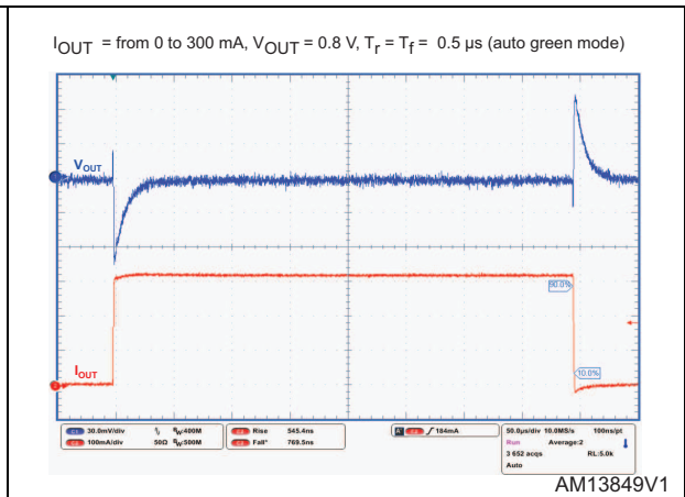
Figure 44. Load transient ( I_{OUT} = 0\text{ to } 300\text{ mA} , auto green mode)
