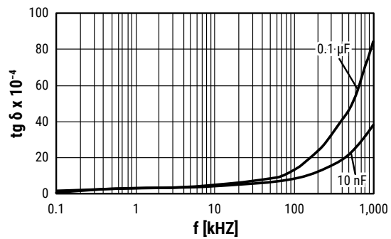
Dissipation Factor vs. Frequency
