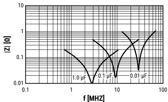
PEN and PPS Impedance vs. Frequency
