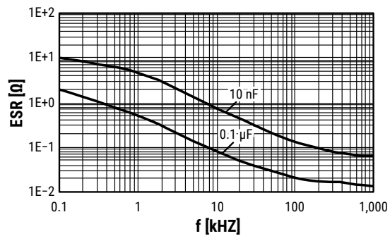
Equivalent Series Resistance vs. Frequency
