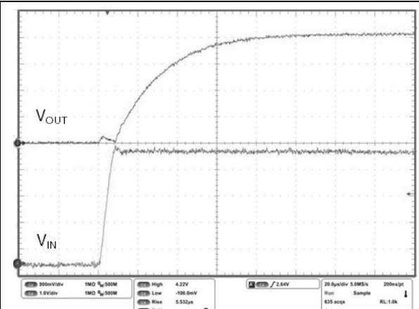
Figure 30. Startup transient
