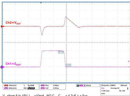
Figure 26: Load transient (VOUT = 1.2 V)
