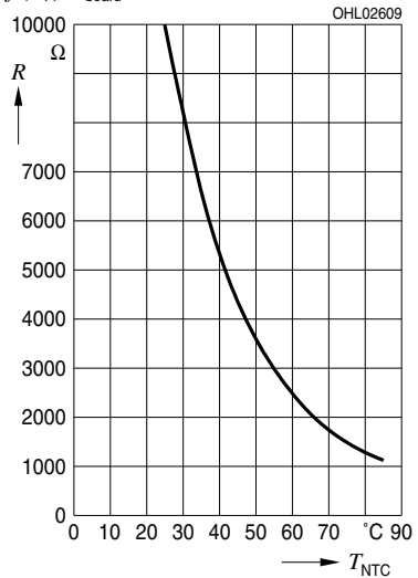
Typische Thermistor Kennlinie (2) 7 Seite 16 Typical Thermistor Graph (2) 7 page 16 I F = f(V F ); T board = 25 °C
