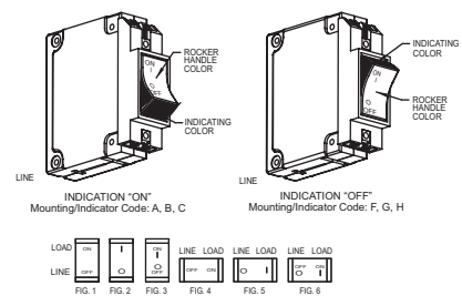
MARKING DETAIL "A" (SEE TABLE)
