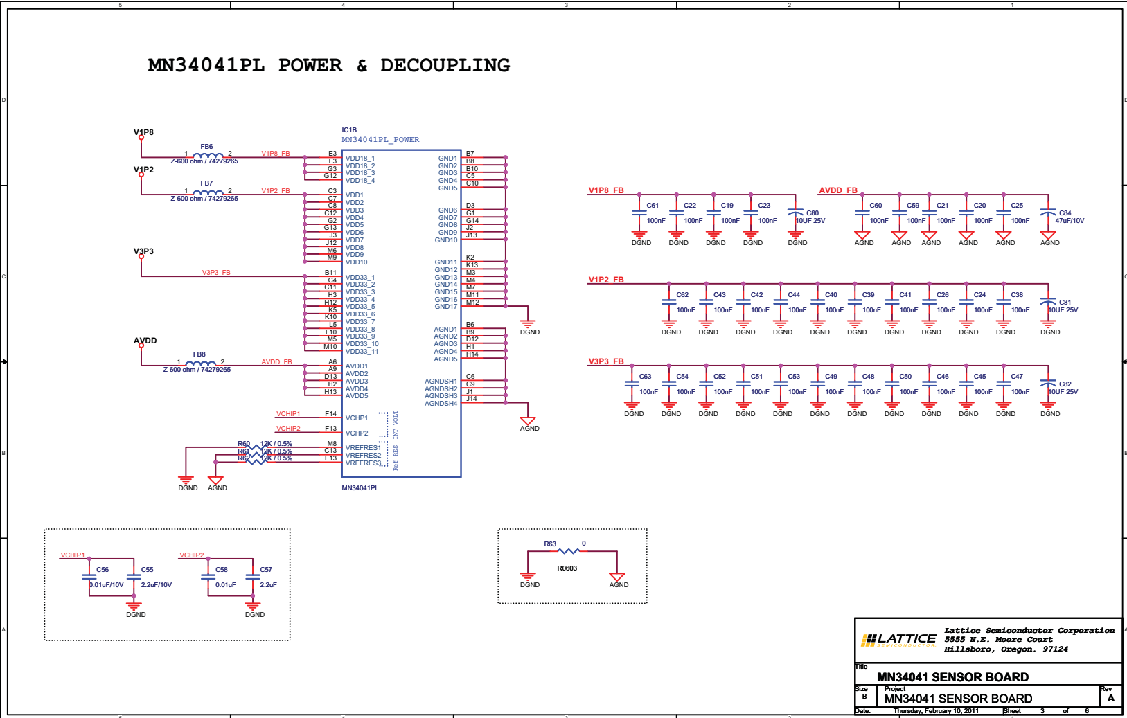
Figure 4. MN34041PL Power
