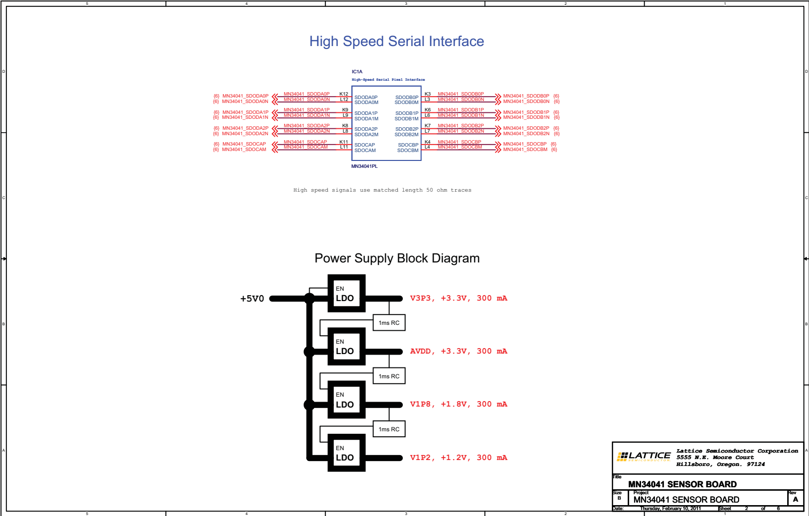
Figure 3. MN34041PL - Serial Interface
