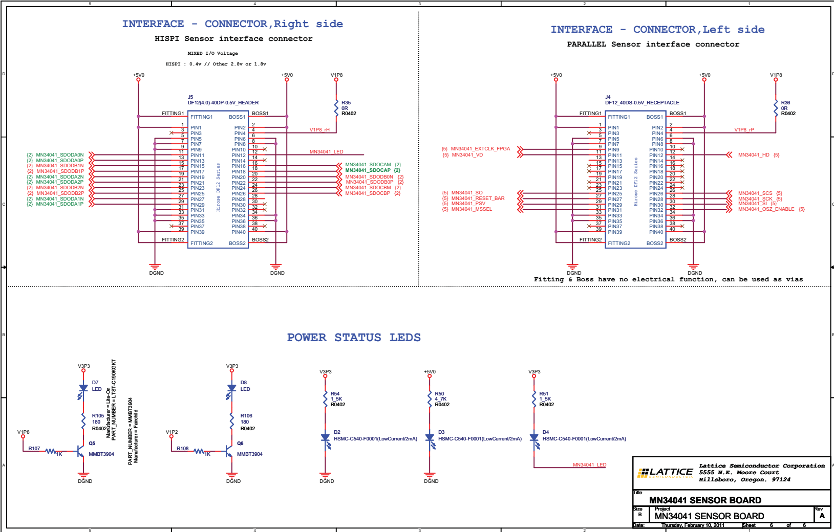
Figure 7. Interface Connectors
