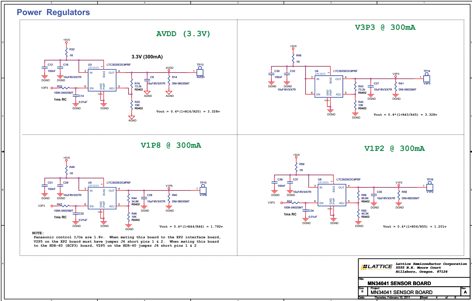
Figure 5. Power Regulators
