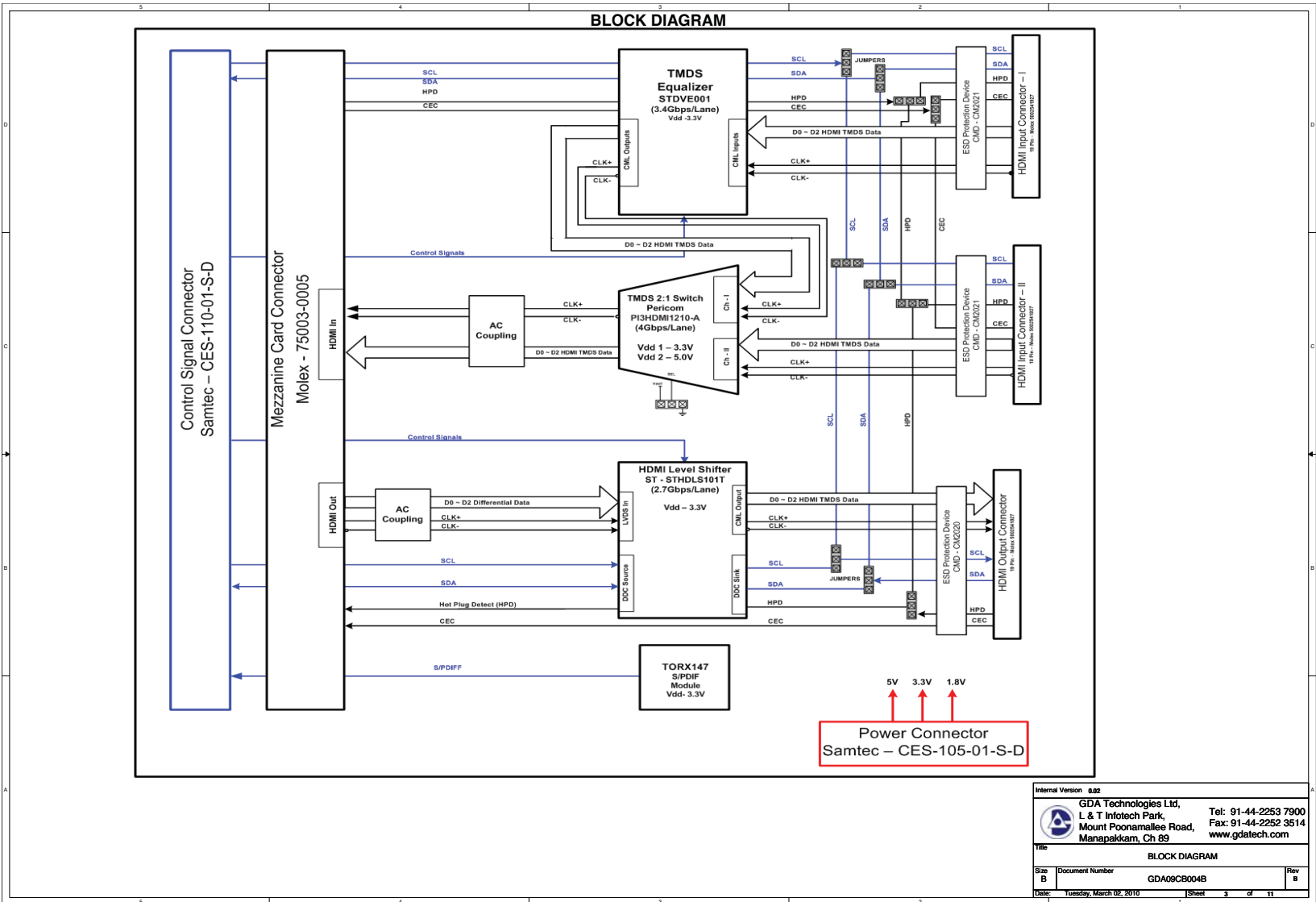
Figure 9. Block Diagram
