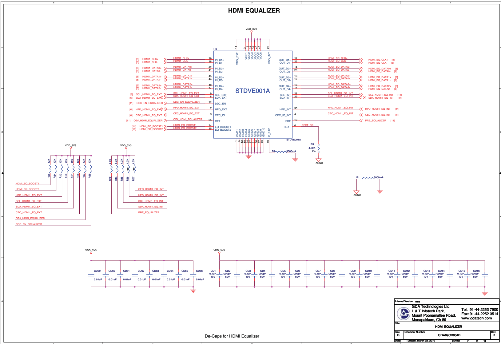
Figure 13. HDMI Equalizer
