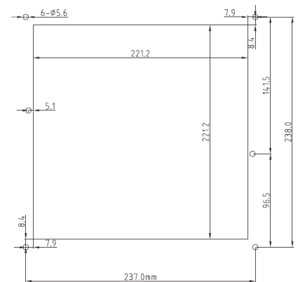
PANEL CUTOUT
