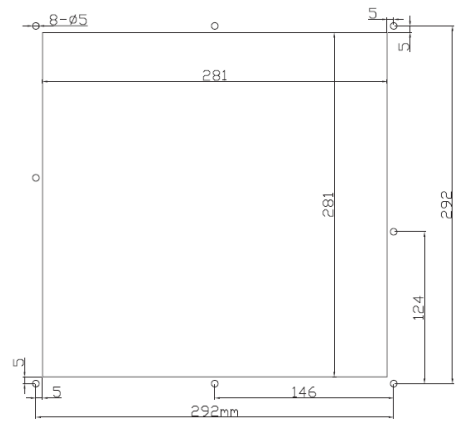
PANEL CUTOUT
