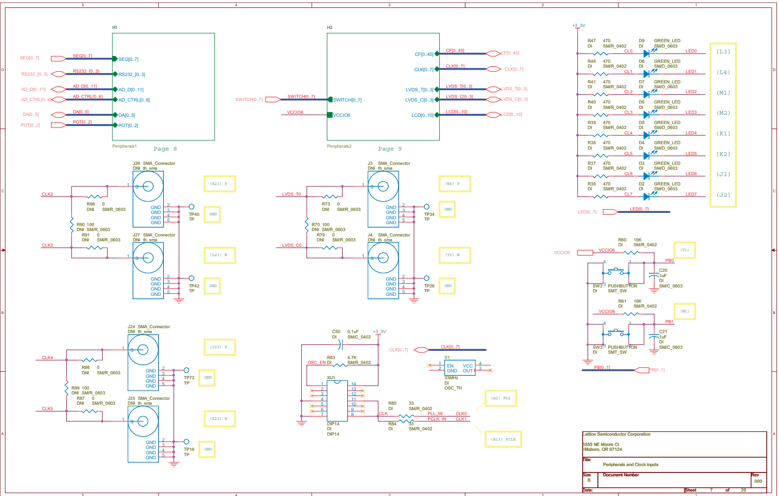
Figure 10. Peripherals and Clock Inputs
