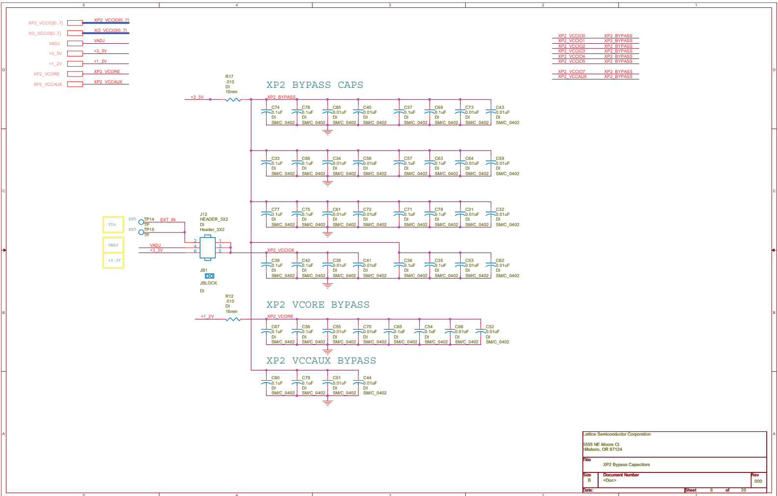
Figure 9. LatticeXP2 Bypass Capacitors
