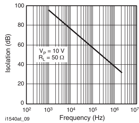
Fig. 10 - Output Isolation
