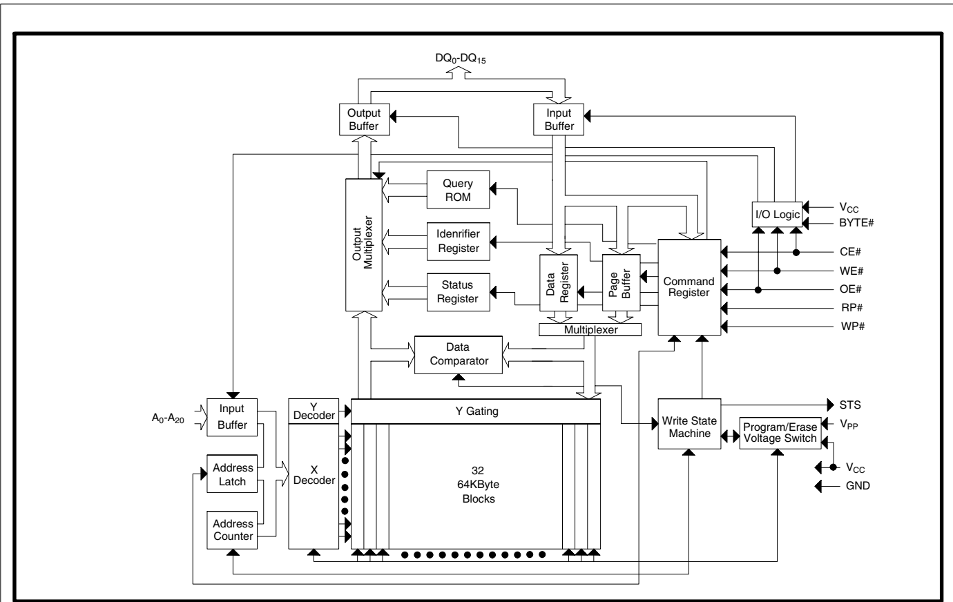
Figure 1. Block Diagram
