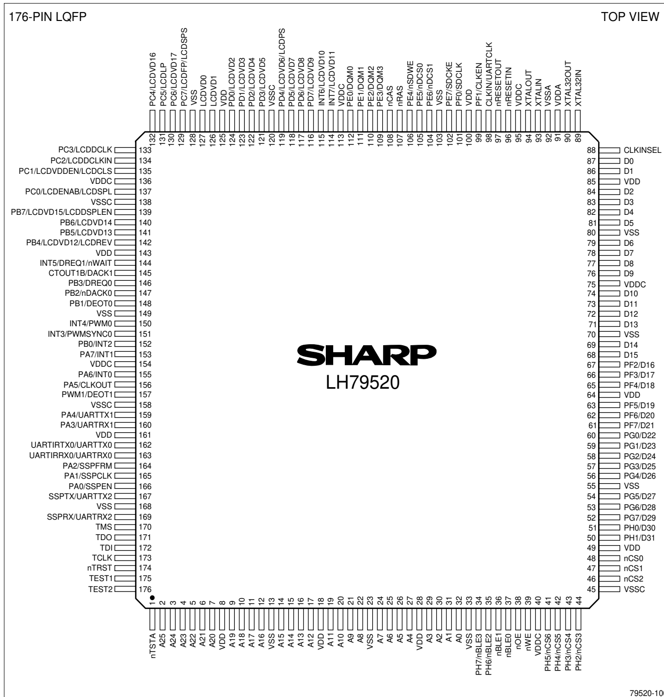
Figure 1. 176-Pin LQFP
