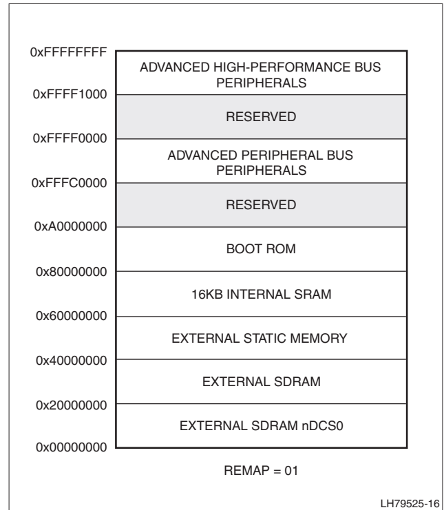
Figure 4. Memory Remap '01'
