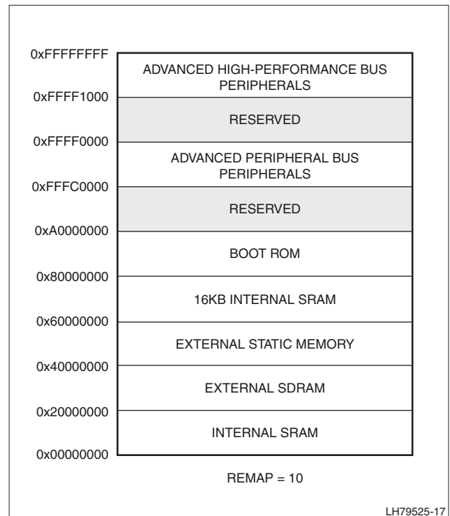
Figure 5. Memory Remap '10'
