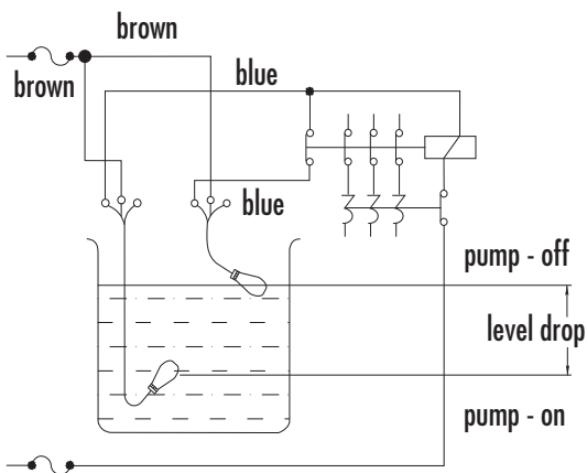
wiring diagram for filling pump
