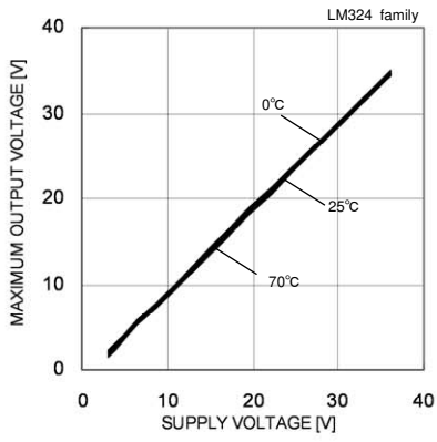
Fig. 28 Maximum Output Voltage - Supply Voltage
