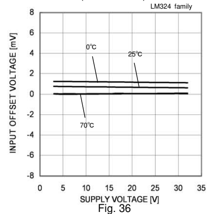
Fig. 36 Input Offset Voltage - Supply Voltage
