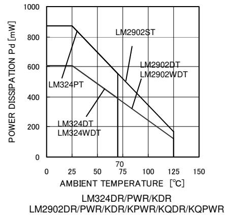
Power Dissipation
