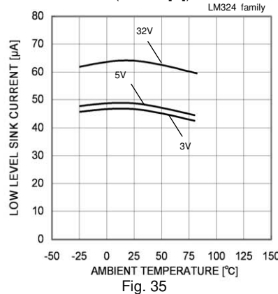
Fig. 35 Low Level Sink Current - Ambient Temperature
