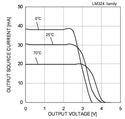
Fig. 30 Output Source Current - Output Voltage
