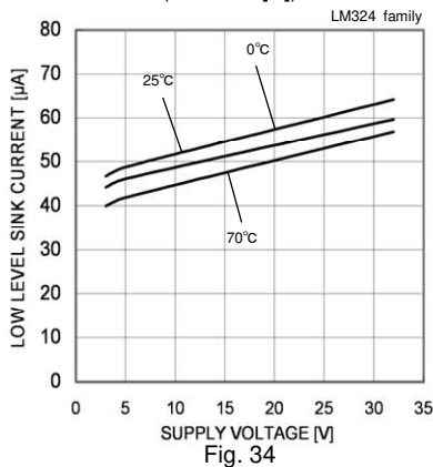
Fig. 34 Low Level Sink Current - Supply Voltage
