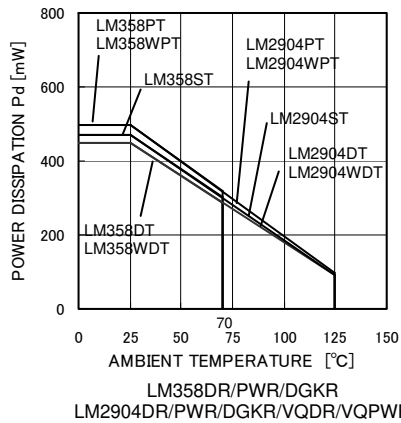
Power Dissipation
