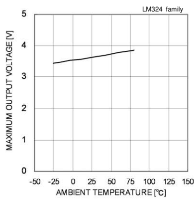
Fig. 29 Maximum Output Voltage - Ambient Temperature
