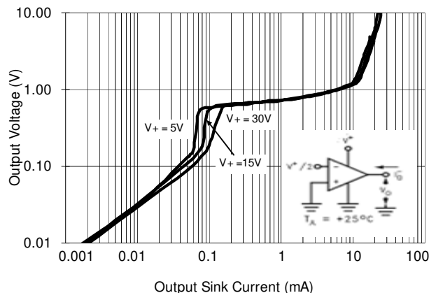
Output Characteristics Current Sinking
