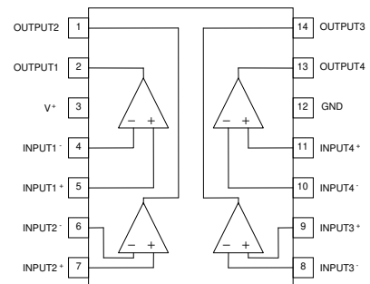
S.O package14
