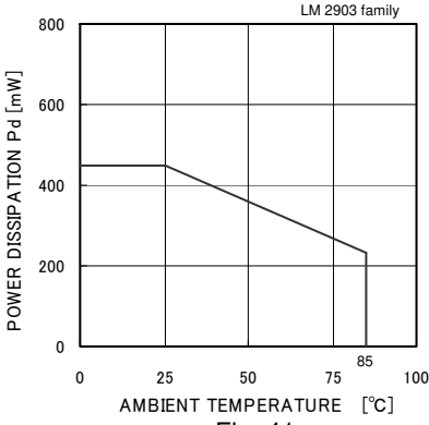
Fig. 41 Derating Curve
