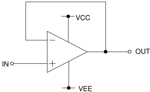
Figure 25. Voltage Follower
