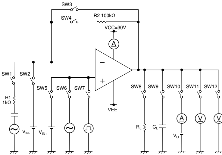
Figure 22. Test Circuit2
