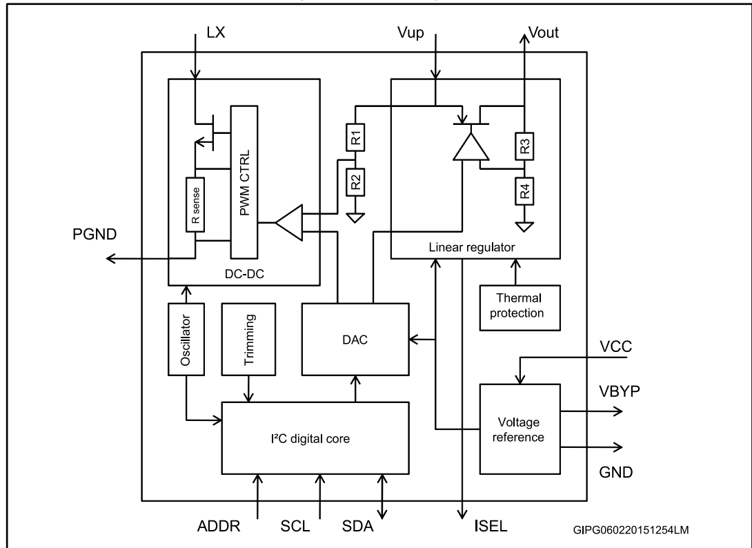
Figure 1: Block diagram
