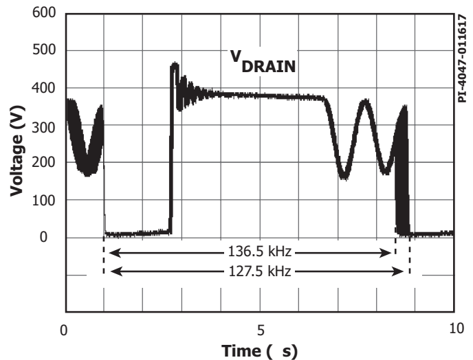
Figure 5. Frequency Jitter.
