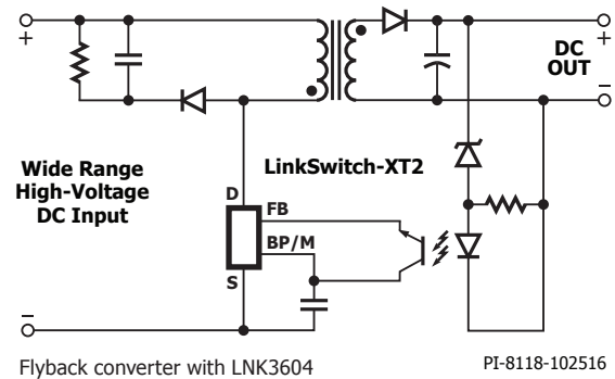
Figure 1. Typical Application with LinkSwitch-XT2.
