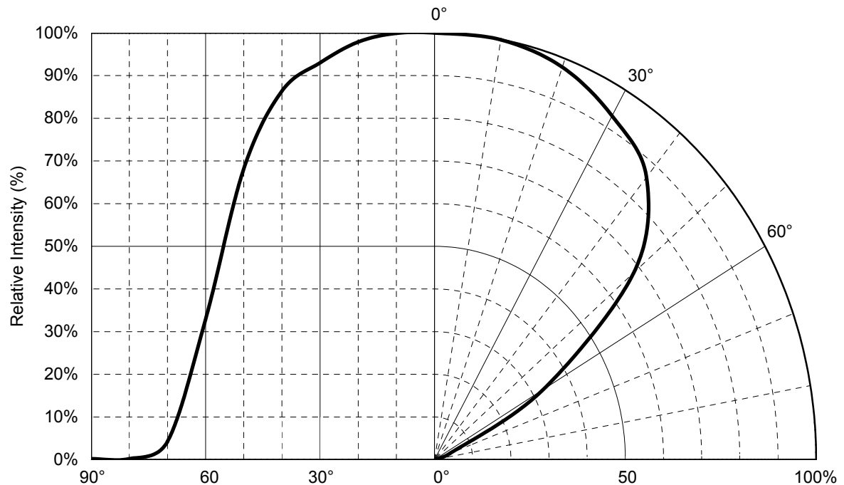
Fig 2. Radiation Characteristics
