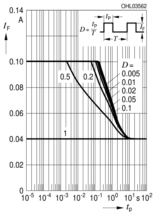
Zulässige Impulsbelastbarkeit Permissible Pulse Handling Capability Duty cycle D = \text{parameter} , T_A = 85\text{ °C} I_F = f(t_p) ; red (1 Chip on)
