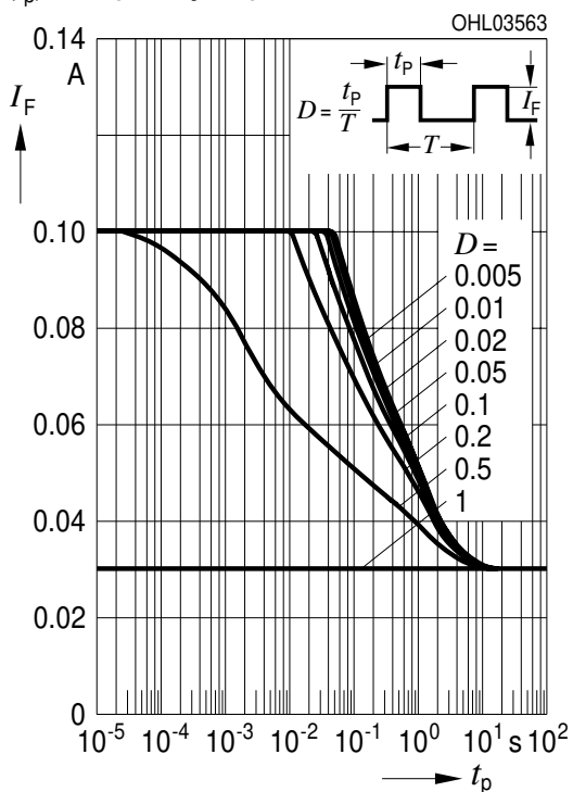
Zulässige Impulsbelastbarkeit Permissible Pulse Handling Capability Duty cycle D = \text{parameter} , T_A = 85\text{ °C} I_F = f(t_p) ; red (1 Chip on)
