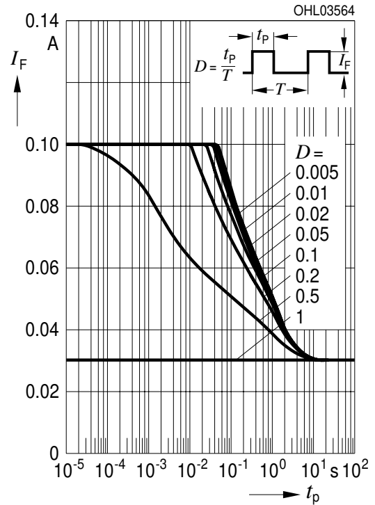
Zulässige Impulsbelastbarkeit Permissible Pulse Handling Capability Duty cycle D = \text{parameter} , T_A = 85\text{ °C} I_F = f(t_p) ; red (3 Chips on)
