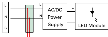
Parallel Connection (for Class II Unearthed)
