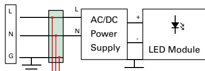
Parallel Connection With LED indicating SPD status - ON (green): SPD is online - OFF: SPD needs replacement
