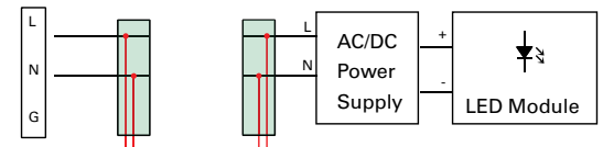
Series Connection (for Class II Unearthed)
