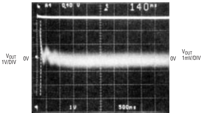
SETTLING TIME TO 1mV, A_V = -1 SUPPLY BYPASS CAPACITORS = 0.1μF + 4.7μF TANTALUM
