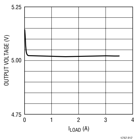
Figure 17. Load Regulation
