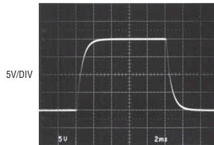
Large-Signal Transient Response G = 1000
