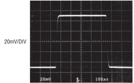
Small-Signal Transient Response G = 10
