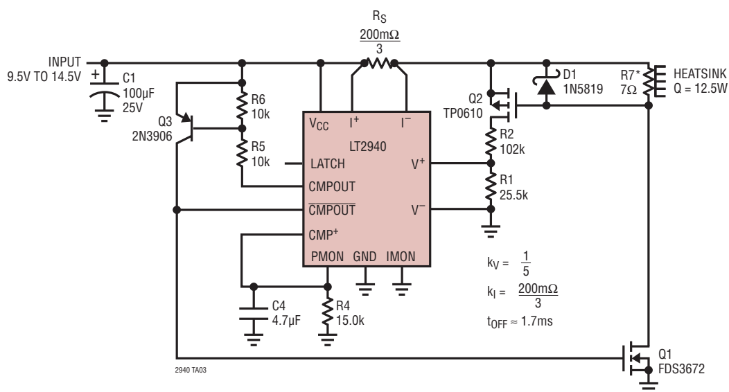
12.5W PWM Heat Source
