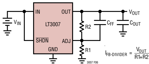
Figure 6. Feedforward Capacitor
