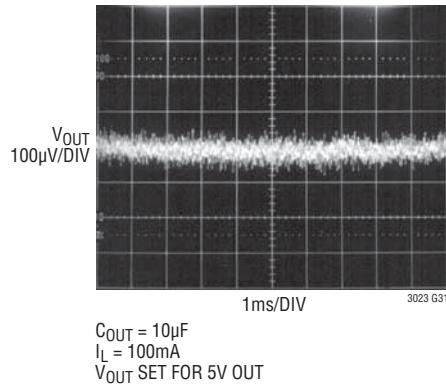
10Hz to 100kHz Output Noise C_{BYF} = 0.01µF
