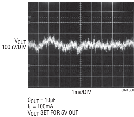
10Hz to 100kHz Output Noise C_{BYF} = 1000pF
