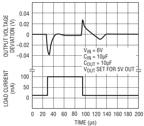
Transient Response C_{BYF} = 0.01µF
