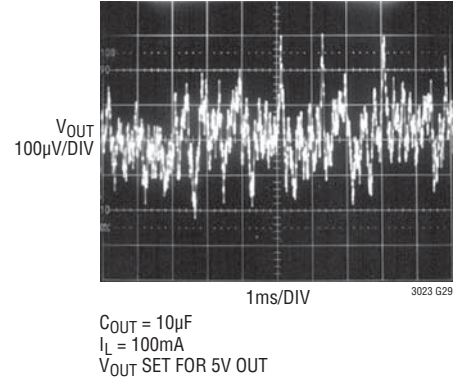
10Hz to 100kHz Output Noise C_{BYF} = 100pF
