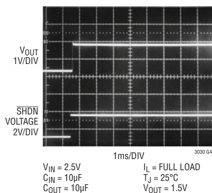
Start-Up Time from Shutdown C_{BYP} = 0\mu\text{F}
